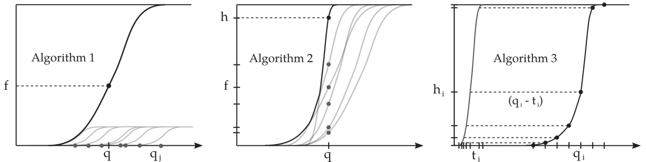
Figure 6: Evaluation of a single CDF at a fixed \phi_l by summing kernel functions centered at M_\theta samples q_j (left); differentiable approximation of the maximum of the CDFs h from M_\phi values of f (center); trapezium rule integration of \hat{D} using N values of q_i , h_i and t_i (right).
